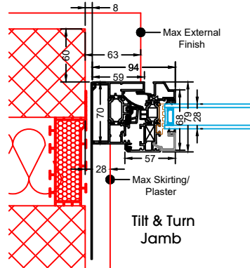
Tilt & Turn Jamb Inc 35mm Add-On
