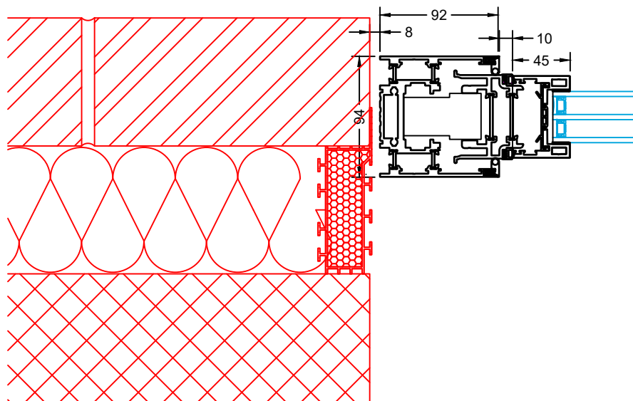
Fixed Jamb in Closed Position
