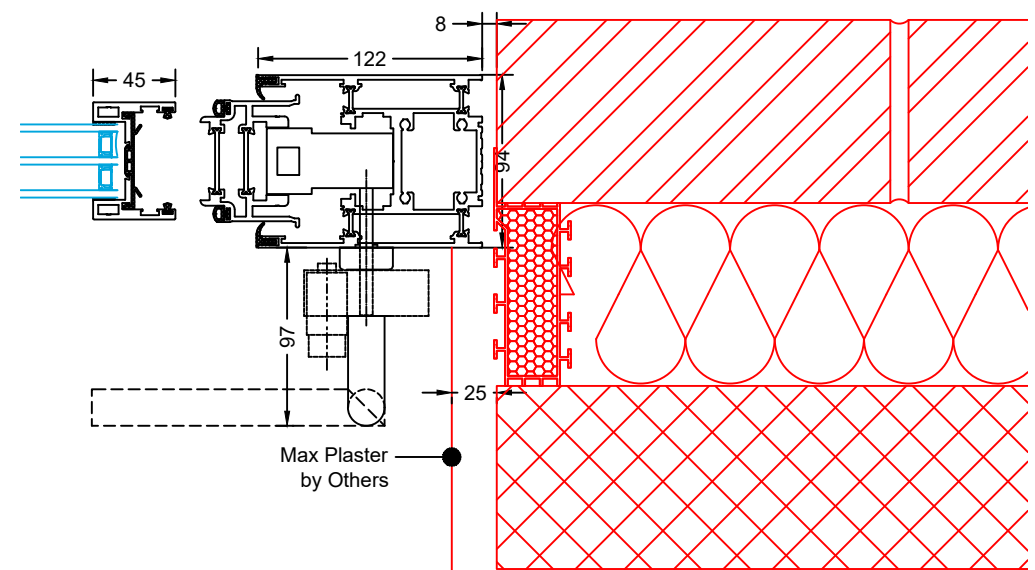
Opening Jamb in Opening Position
