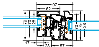
Tilt & Turn Fixed Mullion
