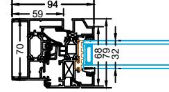
45mm Glass Unit
