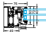
40mm Glass Unit
