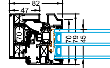
45mm Glass Unit
