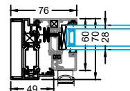
32mm Glass Unit
