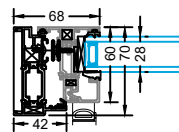
32mm Glass Unit
