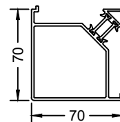
90° Corner Post
