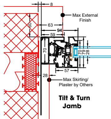
Tilt & Turn Jamb Inc 30mm Add-On
