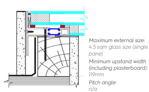
Flush walk-on cross section
