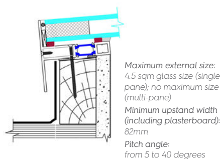
Rooflight cross section
