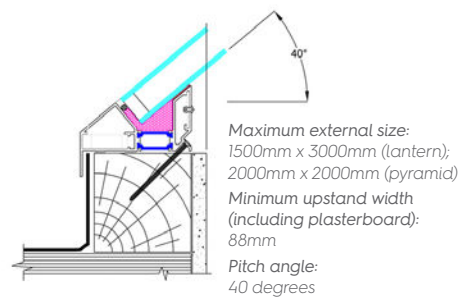
Lantern cross section
