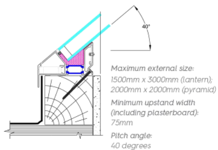
Lantern cross section
