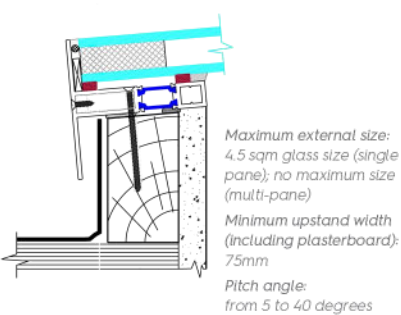
Rooflight cross section
