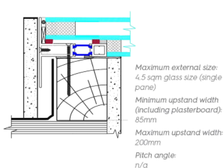
Walk-on cross section
